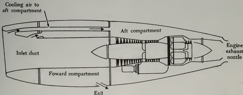
FIGURE 6-48. Typical engine nacelle cooling arrangement.
